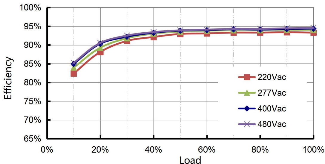
Efficiency vs. Load (C14A)
