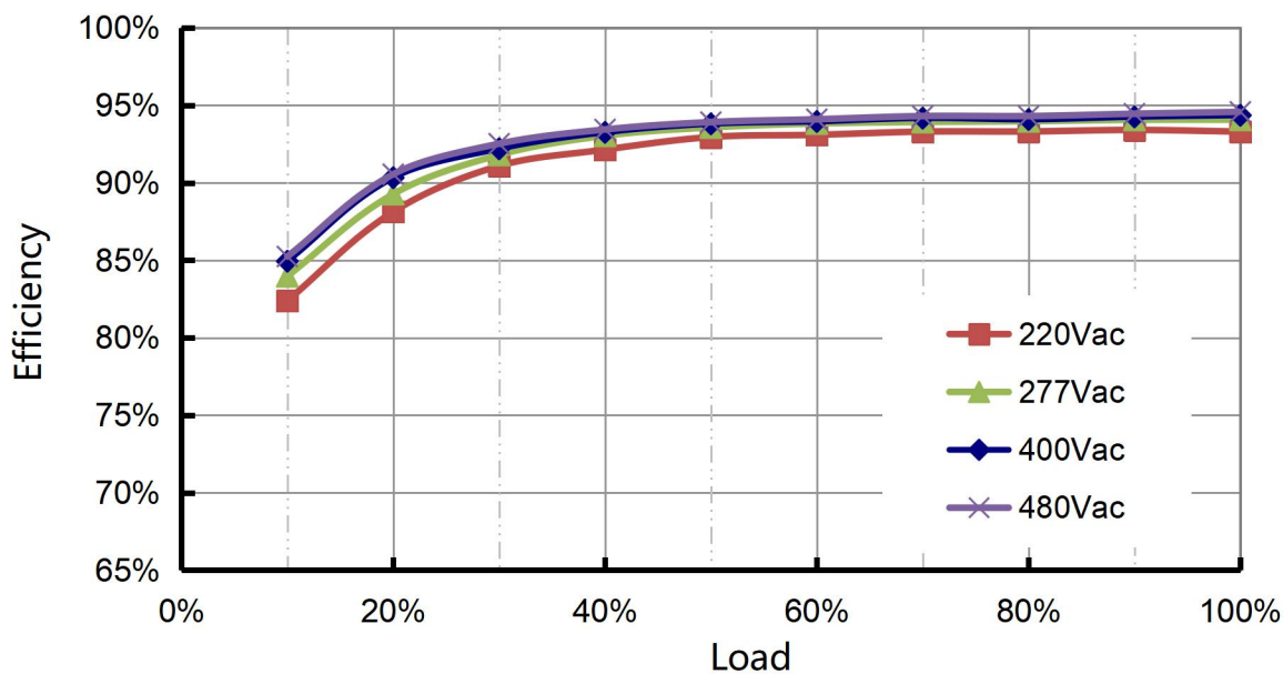
Efficiency vs. Load (C600)
